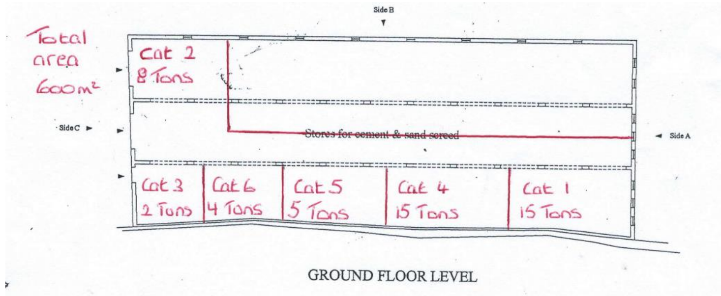
Fig. 2.1: Site Layout showing the permitted facility for the carrying out of the activities specified in condition 1.1.1. The extent of the site boundary is indicative and shall not be used for interpretation purposes.
